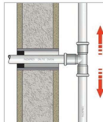
Figure 50c - Creation of expansion spaces
