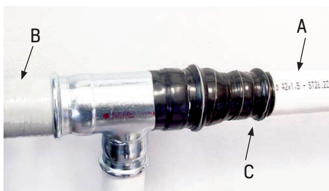
Figure 44 – Protection against external corrosive materials:
