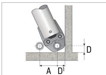
Figure 46 – Minimum distances and space requirements
