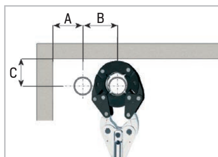
Figure 49 – Minimum distances for chains / collars
