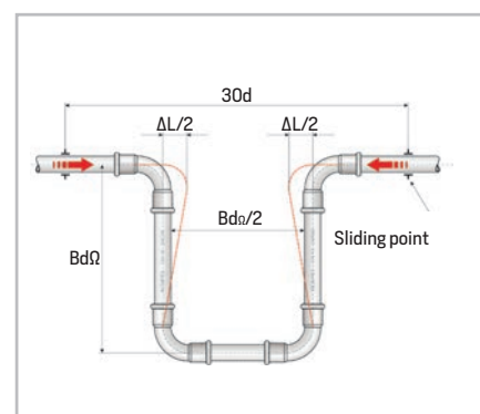
Figure 53 - U-bend Bd\Omega = Bd / 1,8
